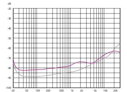
THD与频率, 消波削波以下 10 dB below clip, 8Ω (Class D) (典型性能测量值)
